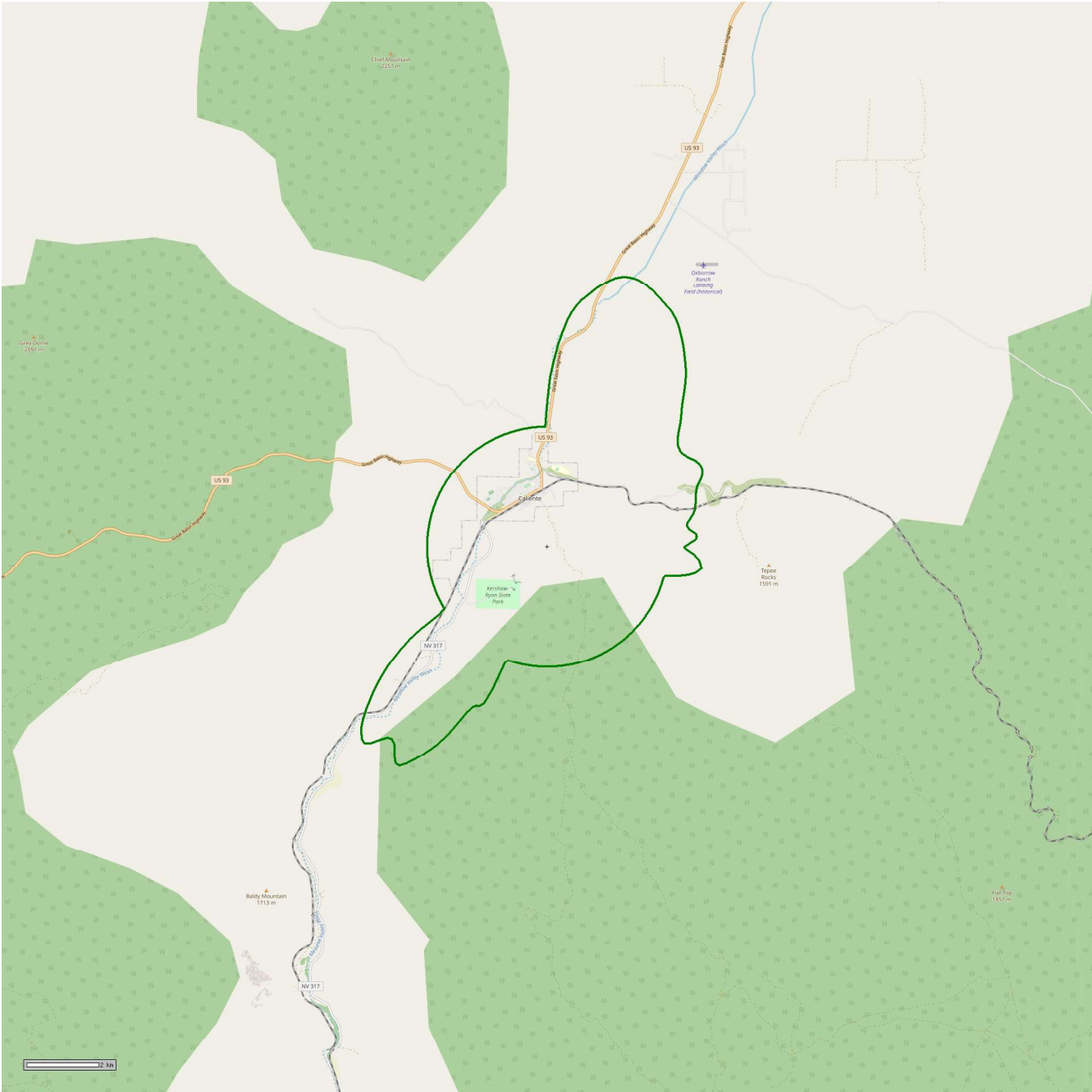
FIGURE 1: The above map depicts the proposed F(50,50) 70 dBu contour that would be produced from the facility described herein. As shown above, the entire community of Caliente, Nevada would lie within the required community of license contour.
