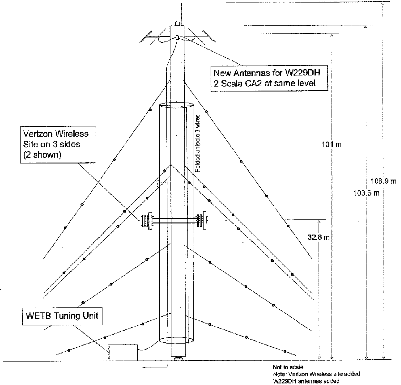
Exhibit 1 WETB, Johnson City, TN Vertical Sketch 24 April 2020
