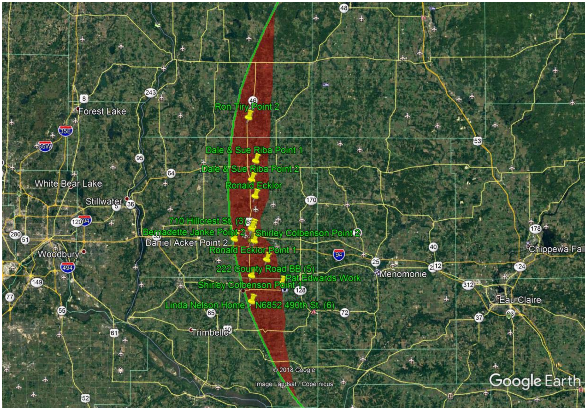
Exhibit 2 Figure 5 Aerial Photo of the WWIB vs W279DD U/D Interference Area with Points of Contention
