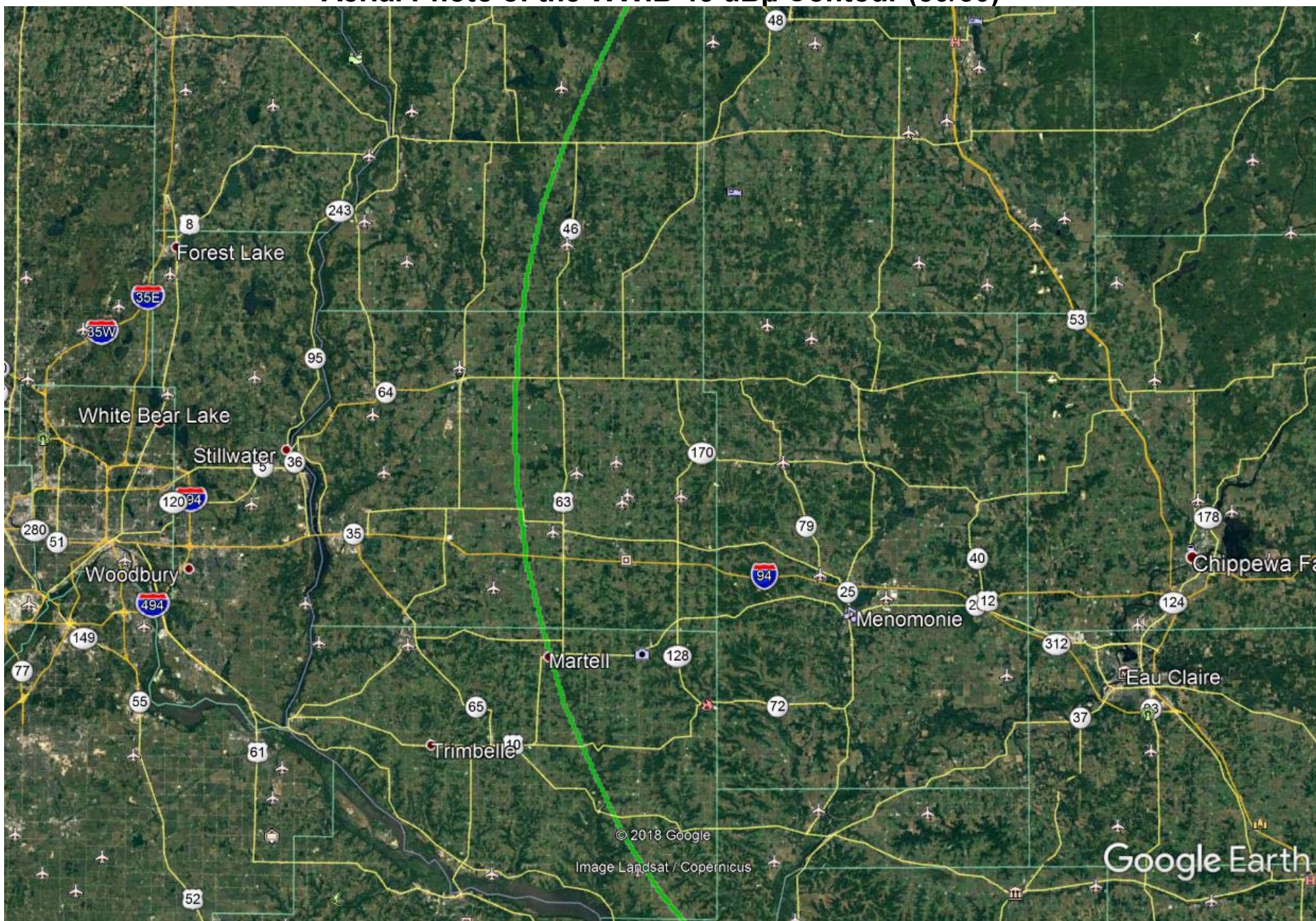
Exhibit 2 Figure 1 Aerial Photo of the WWIB 45 dB \mu Contour (50/50)
