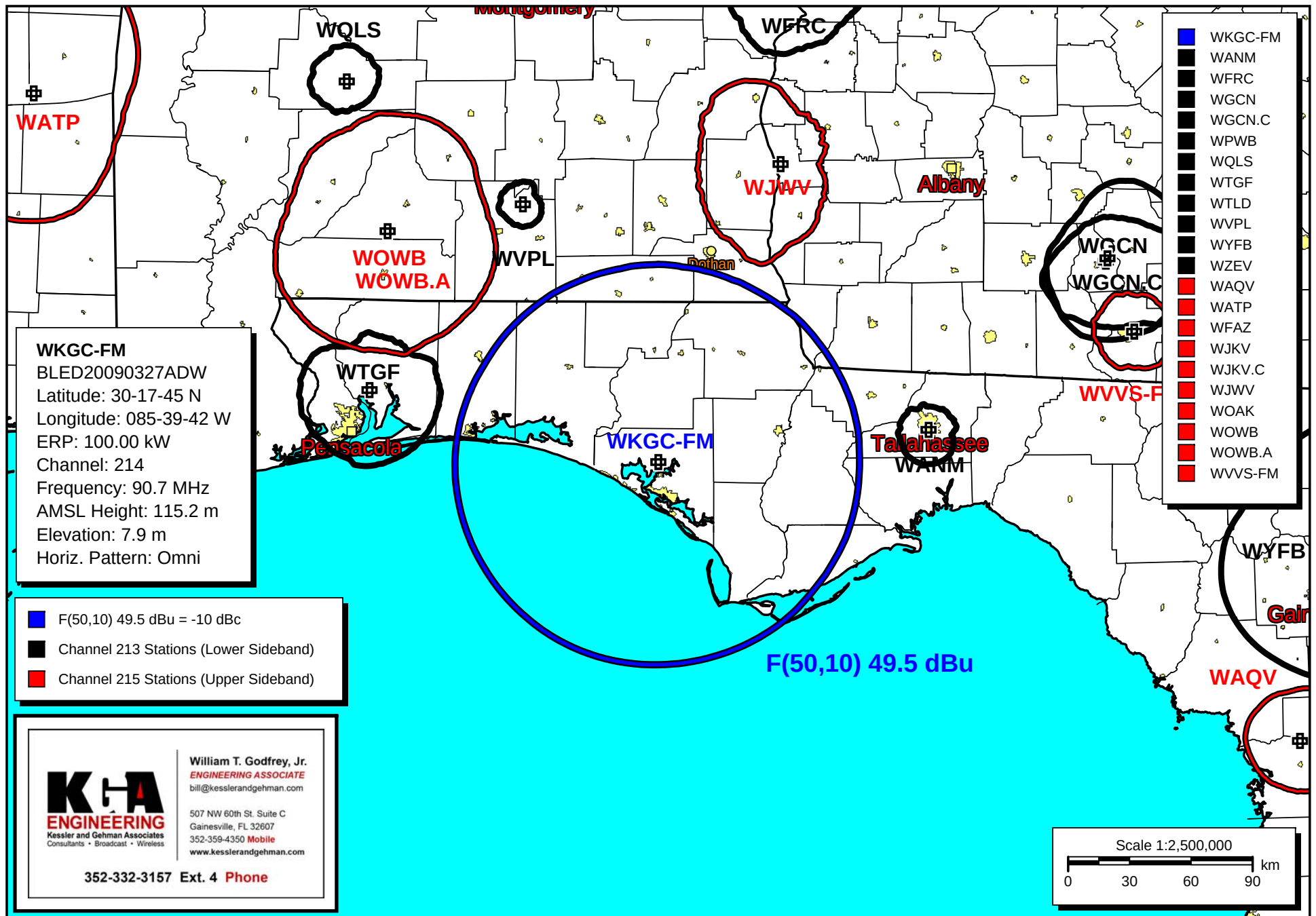
Maximum Permissible FM Digital ERP Study (-10 dBc)
