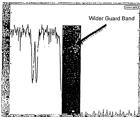
Figure – 11, Single Channel Only Pink Noise, SSBSC
