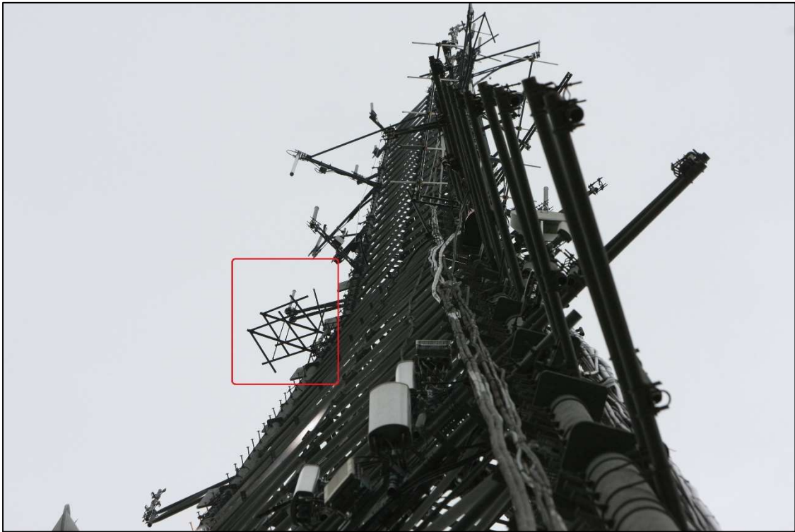
W221DG transmit antenna at licensed height (90m AGL, overall structure height 137.2m)
